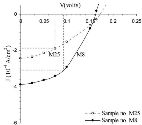
Fig.11. Photovoltaic plots of two typical heat treated ITO-(n)CdSe junctions of different doping concentrations [ N_d = 7.32 \times 10^{16} cm ^{-3} (M8); N_d = 3.03 \times 10^{15} cm ^{-3} (M25)] at room temperature.
