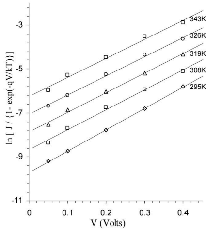
Fig. 8. \ln [J/(1-e^{-qV/kT})] vs V plots of a typical ITO/(n)CdSe junction (M8) in dark at different temperatures.
